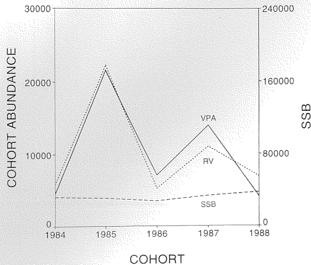
Fig. 1. Gadus morhua . Trends in cohort abundance and spawning stock biomass (SSB, in t) for Georges Bank cod through the 5 yr study period. As independent measures of cohort abundance, the VPA numbers at age 1 ( \times 10^3 fish) and the first principal component of a scaled RV index show similar trends, although neither reflect SSB
