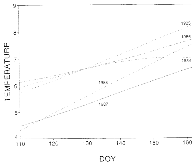
Fig. 5. Daily temperature ( ^{\circ}\text{C} ) time series for waters of 30 to 50 m depth on the northeast cap of Georges Bank for the years 1984 to 1988, reconstructed from non-daily measurements (see text)
