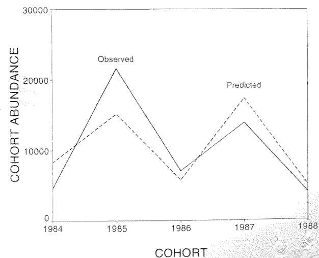
Fig. 8. Gadus morhua . Correspondence between observed cohort abundance ( \times 10^3 fish) from VPA and that predicted from spawning stock biomass after adjusting for growth-related interannual differences in cumulative mortality in the larval and juvenile stages. The correspondence is significant ( p < 0.05 ), while that with unadjusted spawning stock biomass (Fig. 1) is not
