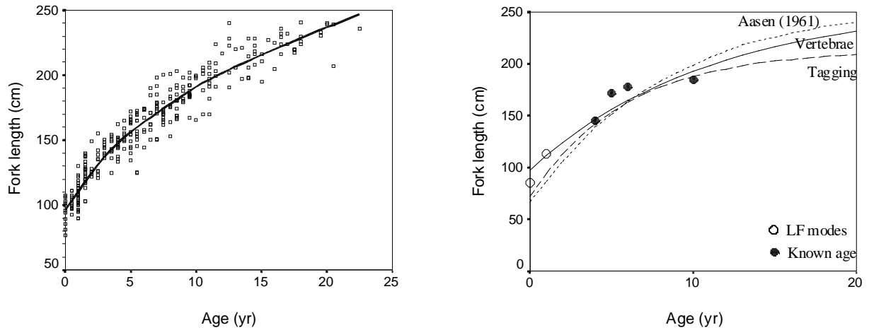
Fig. 6. (Left) Porbeagle growth curve based on vertebral ring counts, fitted with a Loess curve. There was no significant difference between the sexes. (Right) Comparison of von Bertalanffy growth curve fit to growth curves based on independent data. Unpublished age data courtesy of L. Natanson and J. Mello, NMFS.
