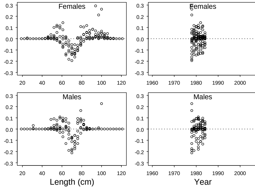
Figure A1.19 (con't). Model 5 ( \alpha=2 ; all data) raw residuals for proportions-at-age.
