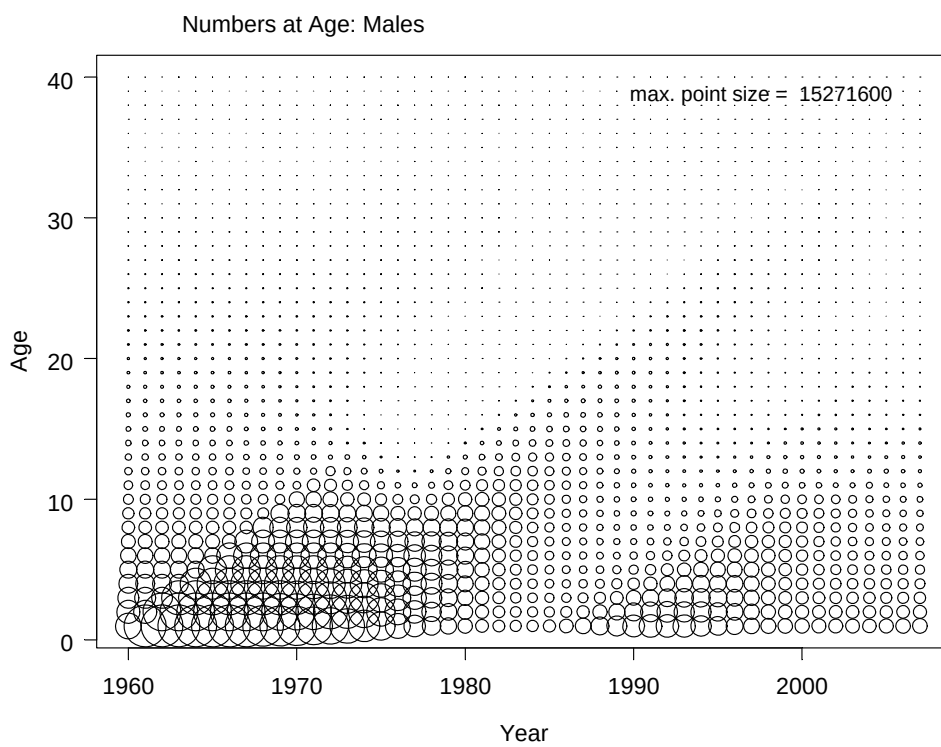
Figure A1.18. Model 5 ( \alpha=2 ; all data) predicted numbers at age.
