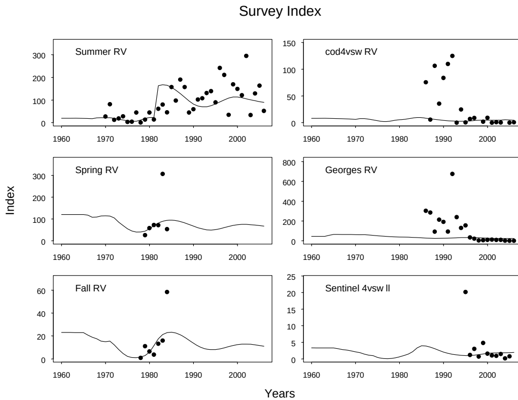
Figure A1.16. Model 5 ( \alpha=2 ; all data) observed and predicted summer RV index.
