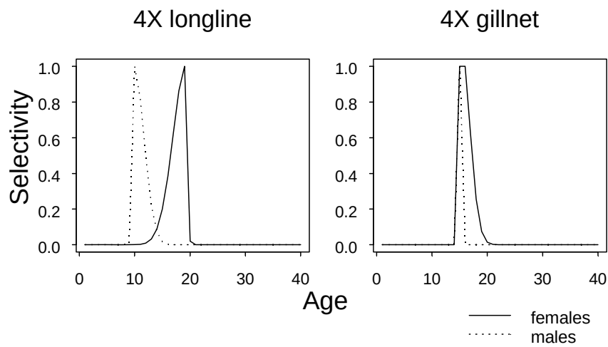
Figure A1.15. Model 5 ( \alpha=2 ; all data) estimated selectivities.
